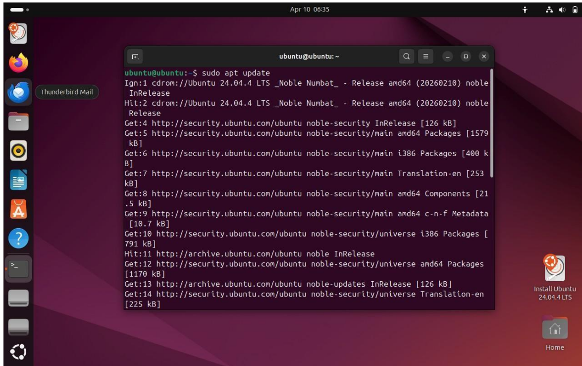
Fig 1.5: Updating package manager
